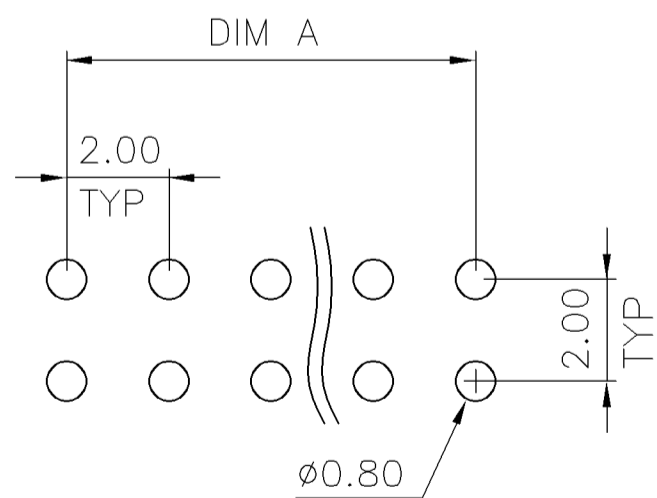
RECOMMENDED PCB LAYOUT (THICKNESS: 1.6mm) (TOP VIEW) (TOLERANCE: ±0.05)
